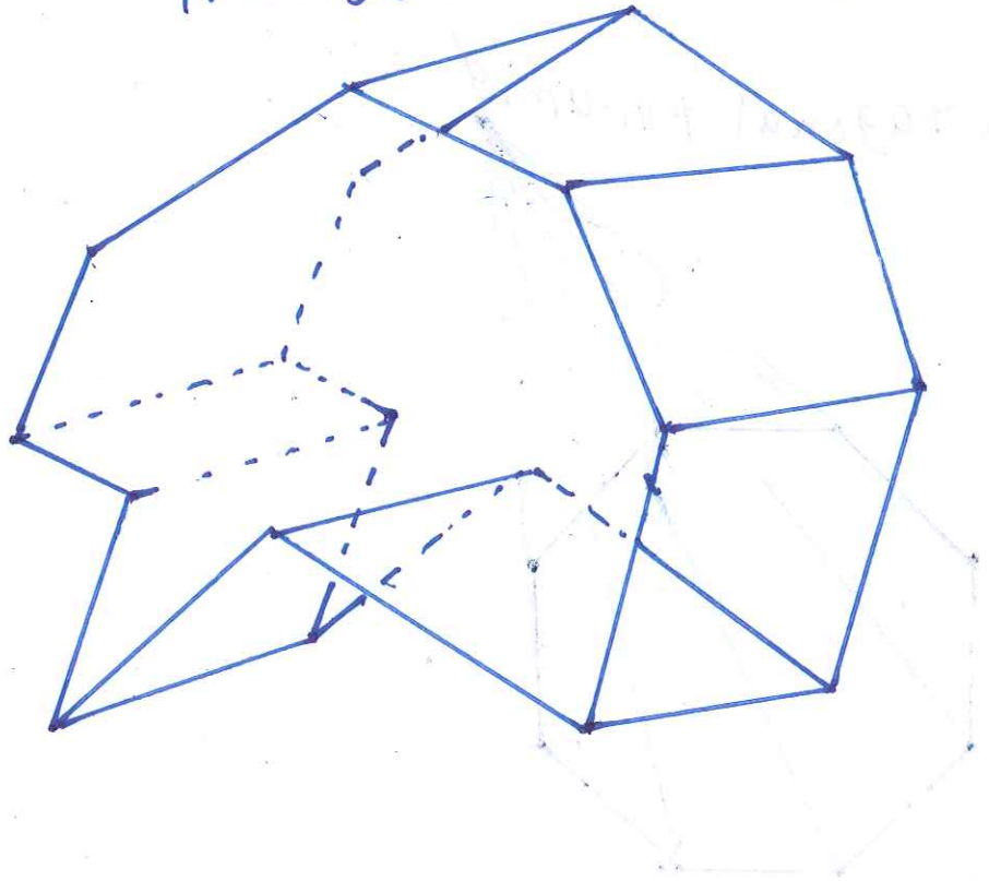
Nonagonal Prism
