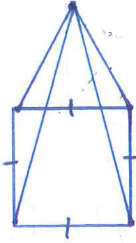
Square pyramid
