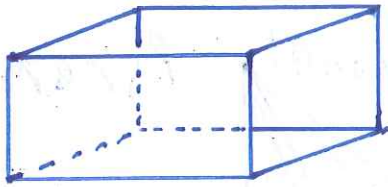
Rectangular Prism
