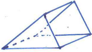
Triangular Prism
