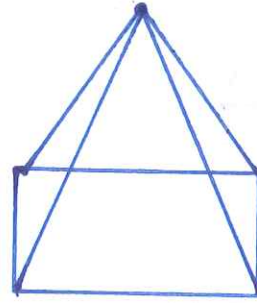
Rectangular Pyramid
