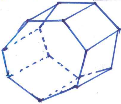
Heptagonal Prism
