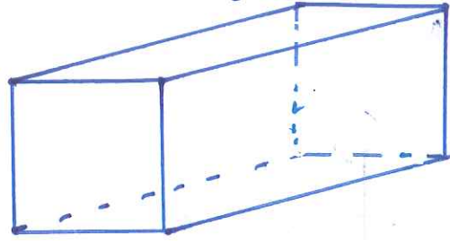
Square Prism
